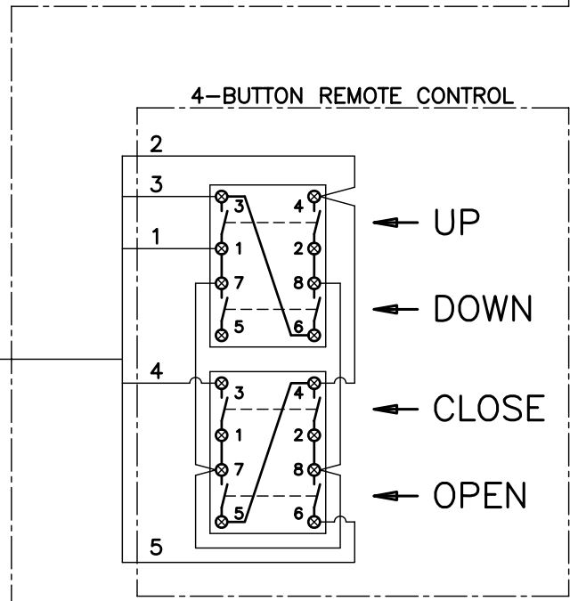
ELECTRICAL WIRING DIAGRAM LDM12BC
