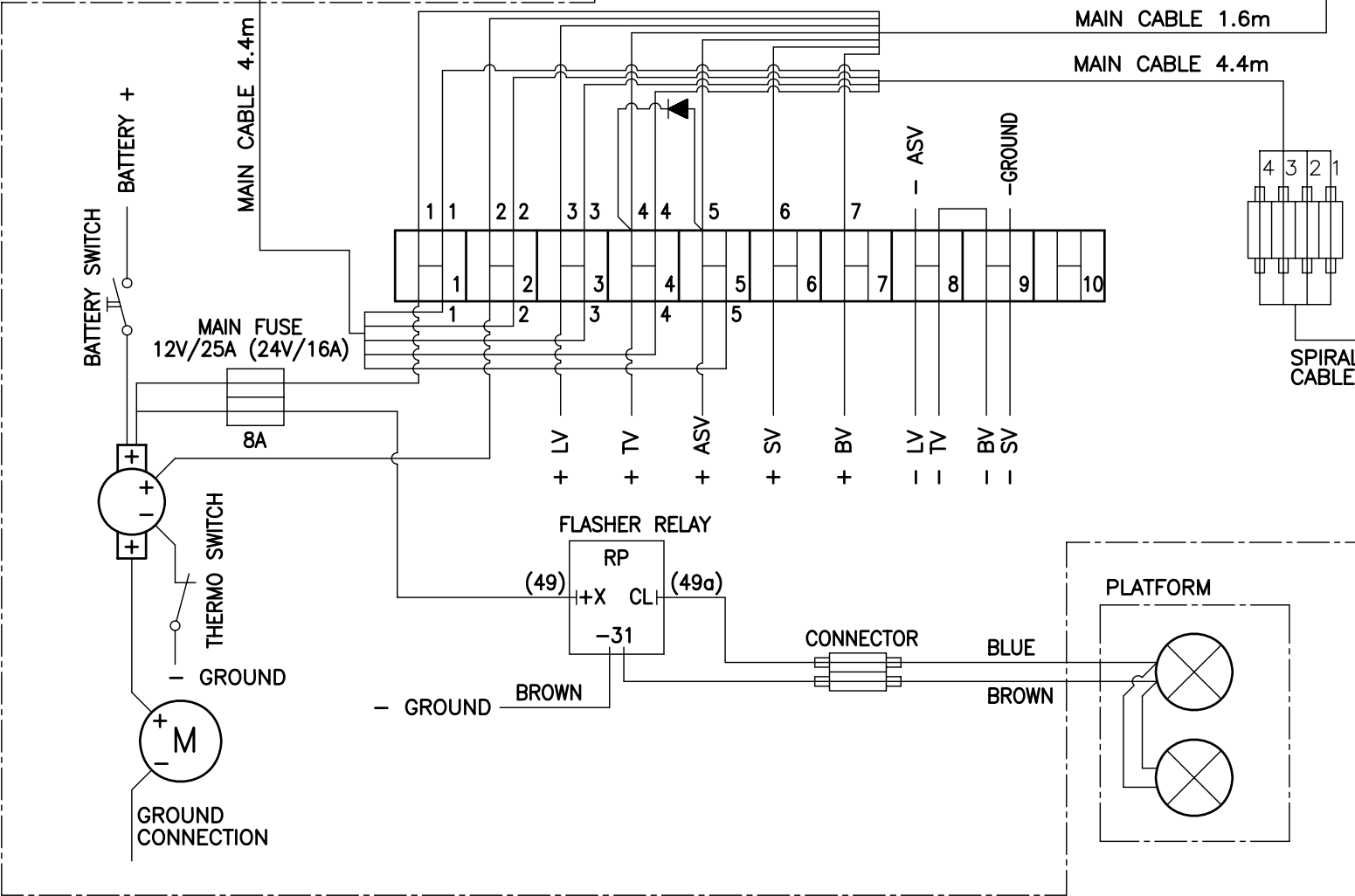
ELECTRICAL WIRING DIAGRAM: LFSMB2BWC
