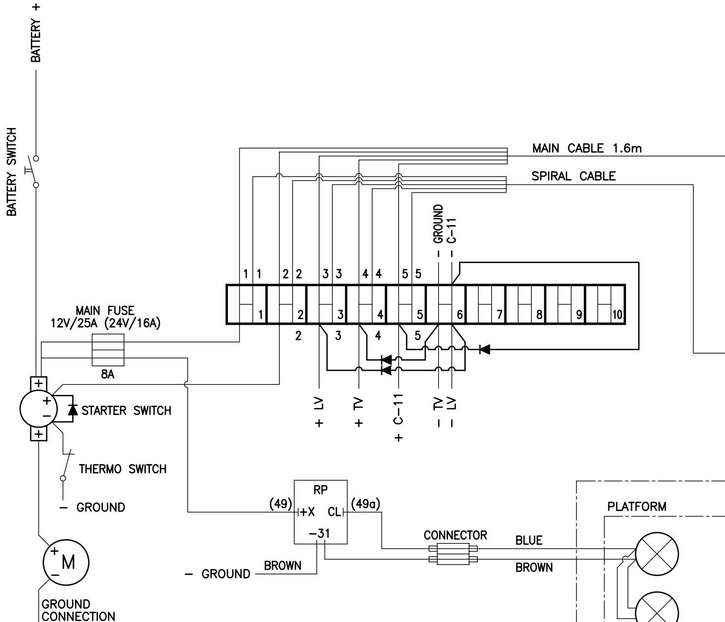
ELECTRICAL WIRING DIAGRAM LSM12BUNC
